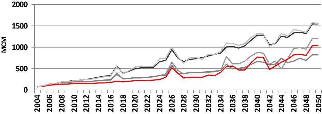
Figure 3: Comparison of unmet water demand (in MCM) in the Jordan basin due to climate change vs. due to socio-economic change, until the year 2050 9
