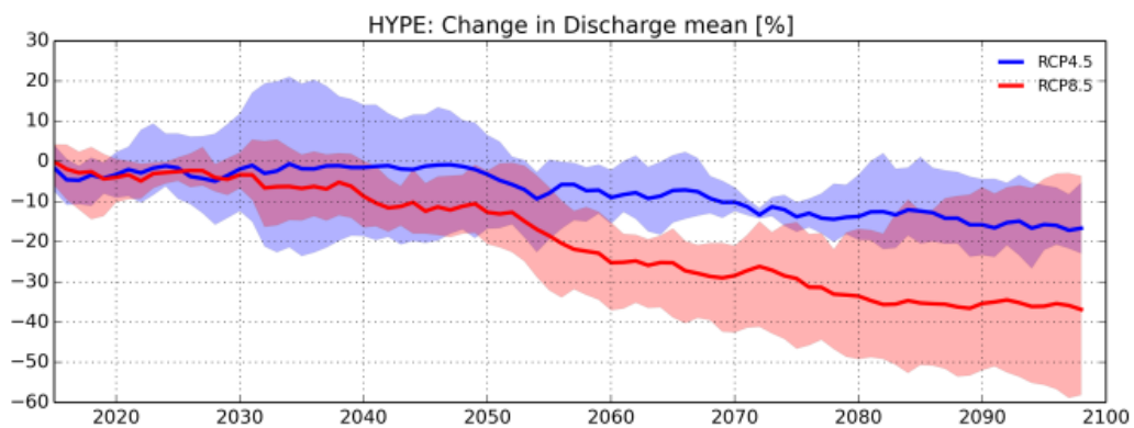
Figure 2: Change in Jordan River discharge as driven by climate change (mean model result and uncertainty range), from RICCAR
