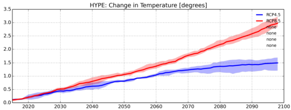
Figure 1: Temperature change for the Jordan River basin for two different climate change scenarios or greenhouse gas concentrations (RCP = representative concentration pathways), from RICCAR
